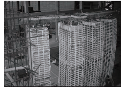
deformation monitoring of large building vibration test
