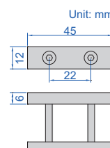
to be used as Go and No-Go gauge
