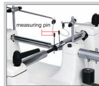
measure pitch diameter of thread
