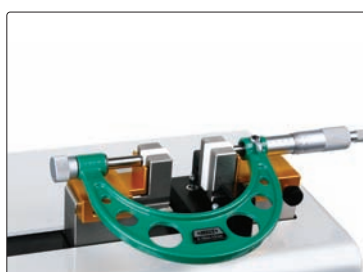
zero setting and calibration of micrometers
