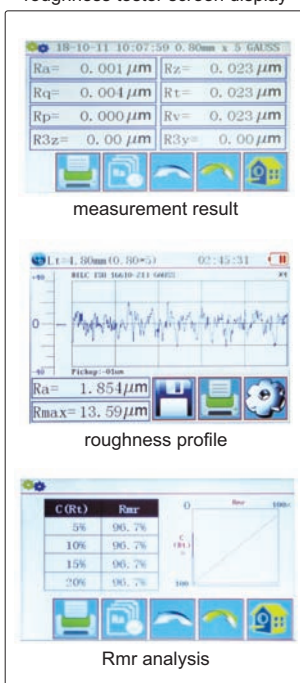
roughness tester screen display
