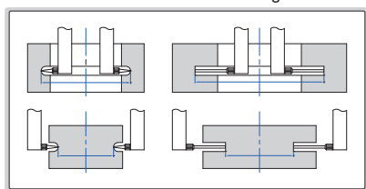
measure internal and external grooves
