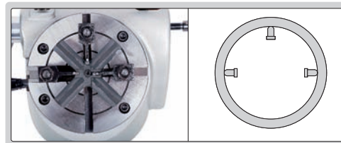
groove probes to measure small internal diameter and internal groove diameter
