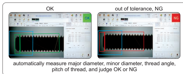
thread measurement
