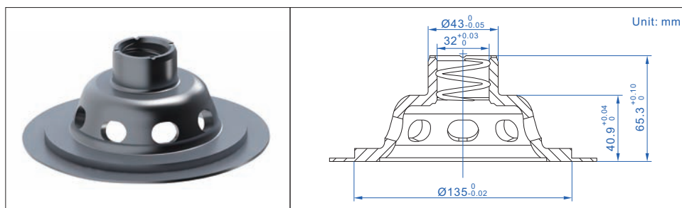
measured workpiece
