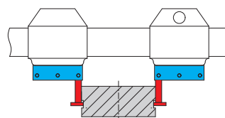
measuring external groove diameter with flat measuring face (depth \leq 2.5\text{mm} )
