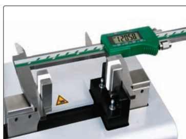
caliper calibration
