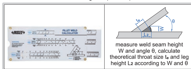
calculating card (included)
