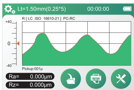
roughness profile
