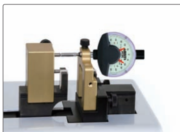
dial comparator calibration
