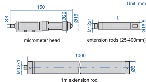
1m extension rod
