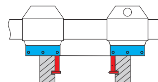
measuring internal groove diameter with spherical measuring face (depth \leq 7.5\text{mm} )
