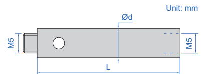
M5 extension rods of styli (mm)
