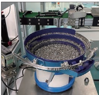
vibratory feeder loading
