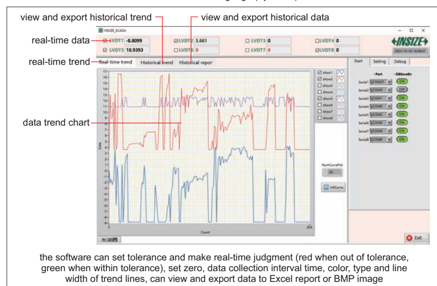
software of linear gauge (optional)
