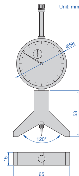
measure depth of keyway
