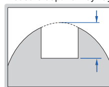
measure depth of keyway
