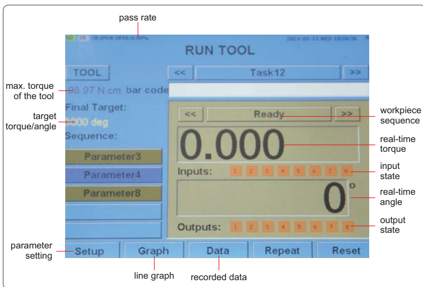
controller (included)
