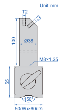
MAGNETIC BASE (mm)
