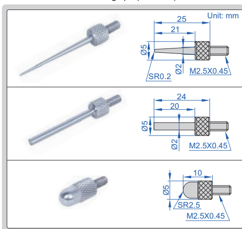
measuring tips (included)
