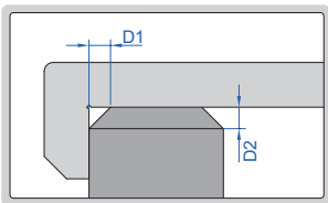
external chamfer
