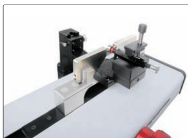
measuring plain plug gauges (manual mode)
