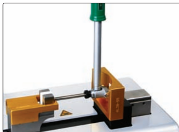
zero setting and calibration of bore gauges
