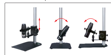
universal stand (included in ISM-PM200SB)
