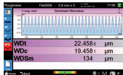
Wdt, WDC, WDSm results
