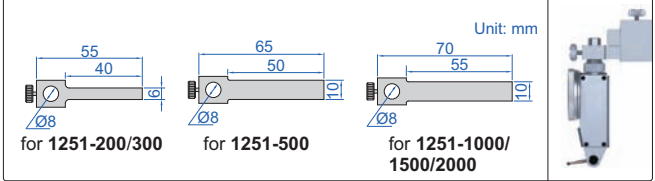
dial test indicator holder (included)
