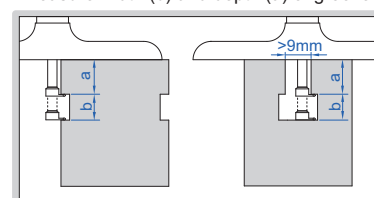
extension rods
