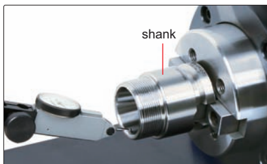
measure radial runout of shank
