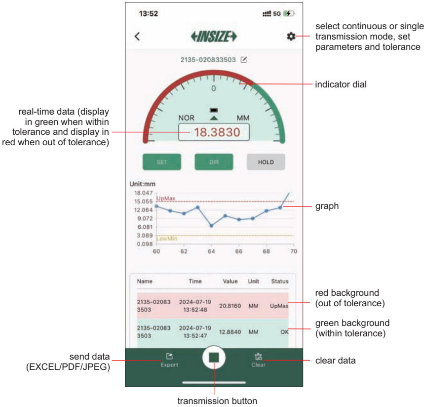
Transmission interface of single digital indicator
