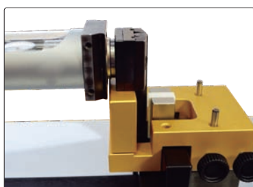
zero setting and calibration of comparison gauges
