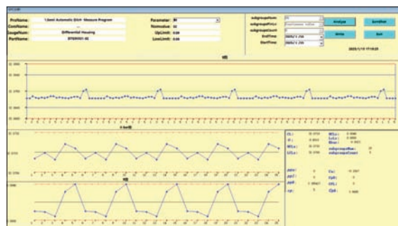
SPC analysis
