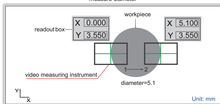
measure length
