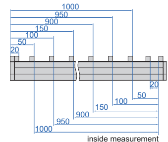
inside measurement
