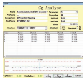
CG analysis
