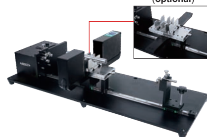
customized fixture (optional)
