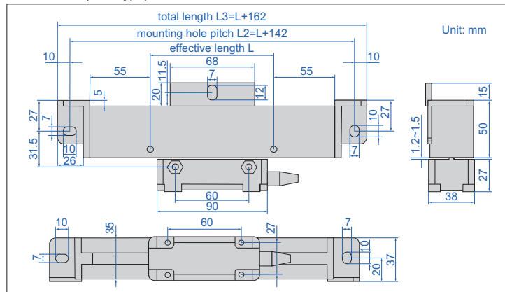
Series ISL-G (thick type)
