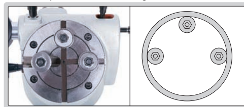
disc probes to measure large internal diameter
