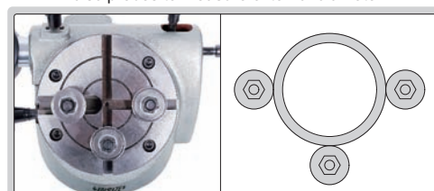
disc probes to measure external diameter
