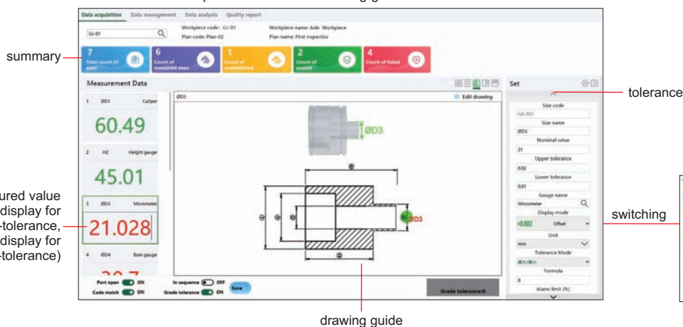
acquisition interface of drawing-guided measurement
